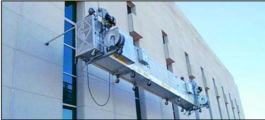
Photo shows how face roller extensions are used to clear window canopies as well as roof mounted light standards located on a lower roof.
