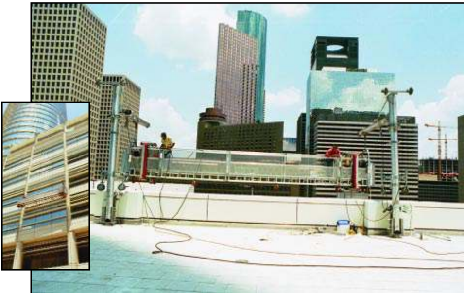
Pro-Bel davits 14'-5" (4.4 m) high with 11'-7" (3.5 m) reach located on 8 th Floor Podium are used to suspend one of a variety of different sized platforms. Inset shows platform traveling down face of Podium.
